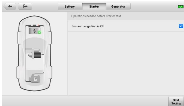
Figure 6-8 Sample Starter Screen 1
